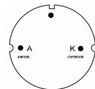
Isolated Pin- Out, Rear View: Anode left; Cathode right
